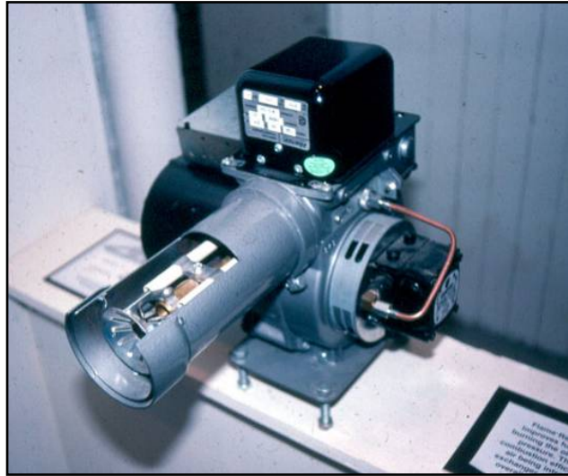
Retention head burner with air blast tube cut away, exposing nozzle and electrodes
