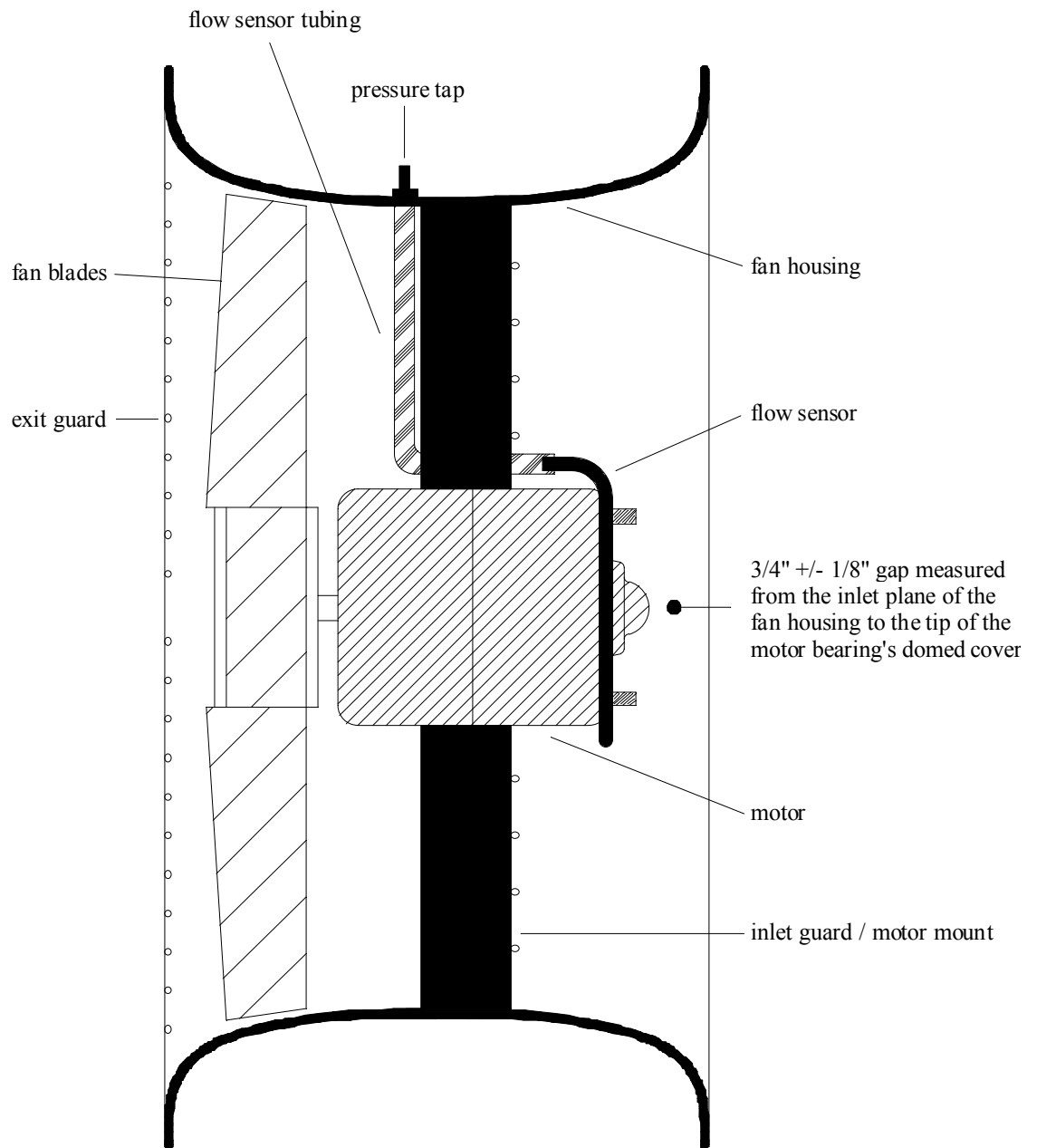
Figure 6: Schematic of Series B Duct Blaster
